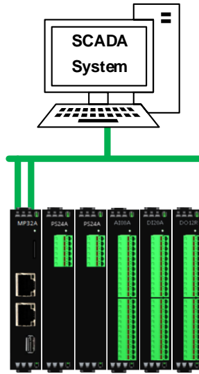
5-Redundant Power Network Redundant
