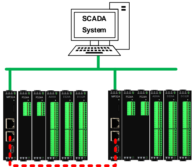
4-Redundant Power Dual I/O Configuration
