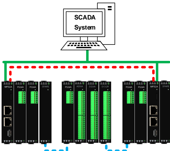
3-Redundant Power Single Share I/O
