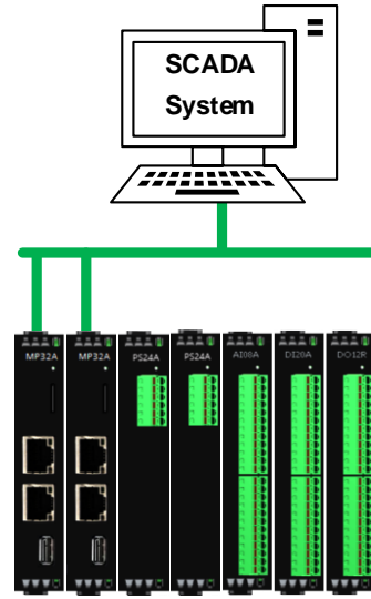
2-Redundant Power CPU Redundant Single I/O Rack
