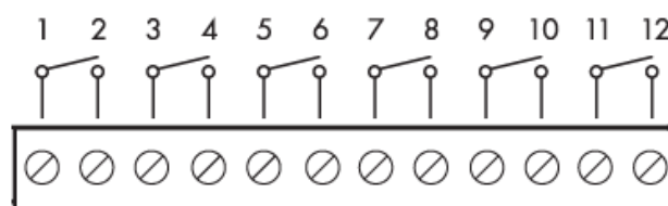
Electrical diagram Relay output
