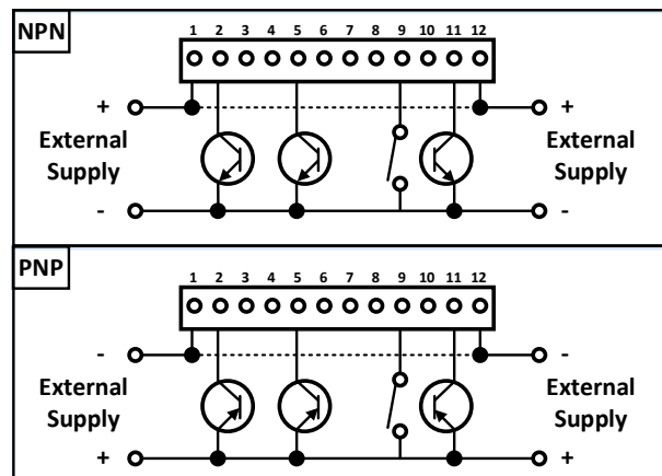
Electrical diagram digital input
